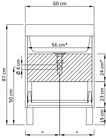
LAVATOIO - LAUNDRY SINK 50x60 - 60x60 con cassettone - with drawer
