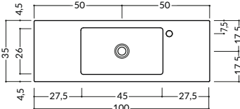
Slim 100 - 100x35 H5 cm - Kg 19
