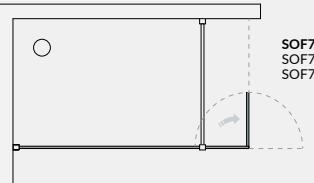
SOF8 reversibile - Reversible SOF8 - SOF8 r  versible
