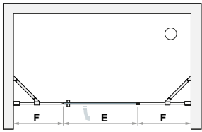
BLP7 DX - BLP7 Rh - BLP7 D
