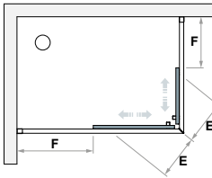
FOA1 reversibile Reversible FOA1 - FOA1 réversible
